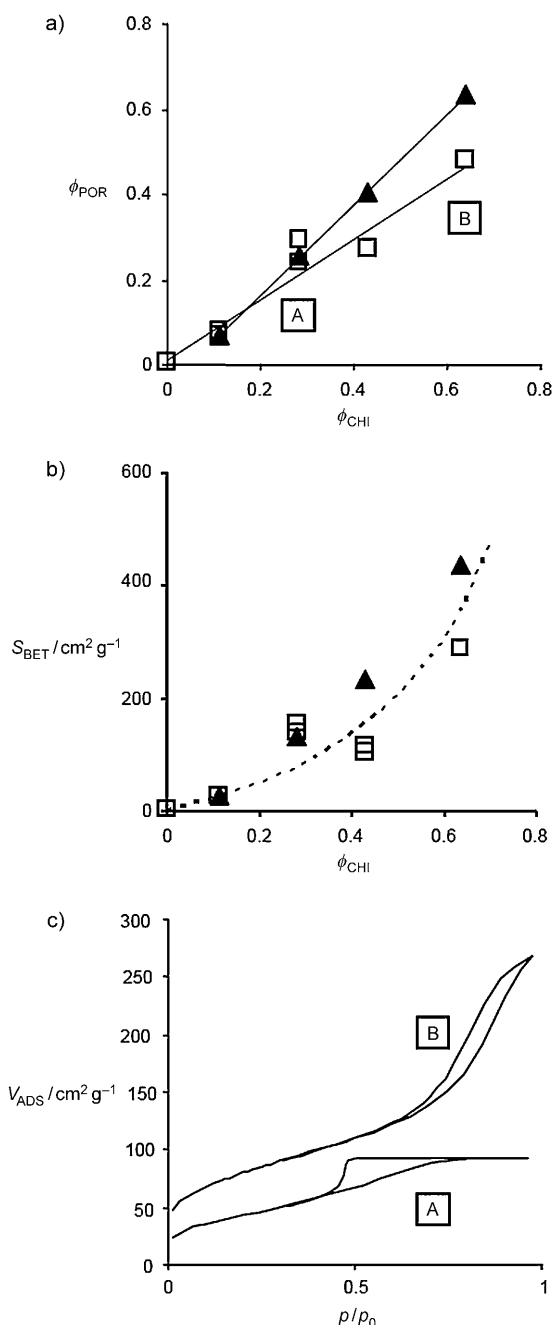
Figure 5. N 2 porosimetry: a) Pore volume fraction \phi_{\text{POR}} as a function of chitin volume fraction \phi_{\text{CHI}} for calcined samples: bulk materials ( \square ) and spray-dried microparticles ( \blacktriangle ). b) Specific surface area S_{\text{BET}} as a function of \phi_{\text{CHI}} for calcined samples: bulk materials ( \square ) and spray-dried microparticles ( \blacktriangle ). The broken line indicates and corresponds to modeled S_{\text{BET}} values obtained using variable \phi_{\text{CHI}} , a density of silica of 2, and dispersed parallelepiped pores of dimensions 10 \times 10 \times 260 \text{ nm}^3 . c) Typical isotherms (adsorbed volume V_{\text{ADS}} versus relative pressure p/p_0 ) obtained for calcined gels, showing a transition from IUPAC type H2 ( \phi_{\text{CHI}} < 0.3 ) to H3 hysteresis loop ( \phi_{\text{CHI}} > 0.4 ). No microporosity is found for any isotherms using the t -plot transformation.
