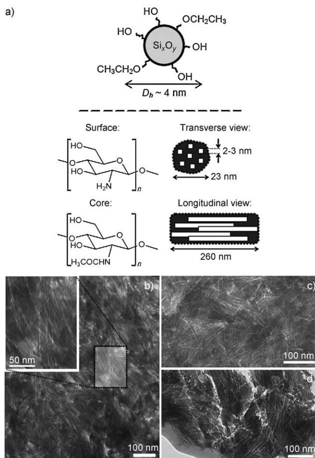
Figure 1. a) Representation of the siloxane oligomers (upper panel), and of the chitin nanorods (core: poly[ \beta -(1 \rightarrow 4)-2-acetamido-2-deoxy-D-glucopyranose]) as bundles of monocrystals with amino groups at their surface (lower panel). The colloid sizes were estimated by DLS and TEM. b–d) TEM analysis: b) bulk nanocomposite ( \phi_{\text{CHI}} = 0.28 ); spray-dried microparticles ( \phi_{\text{CHI}} = 0.28 ) before (c) and after (d) calcination (porous replicas).
